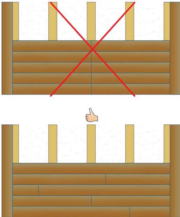
FIGURE 17 • Positioning of lengths and joints
